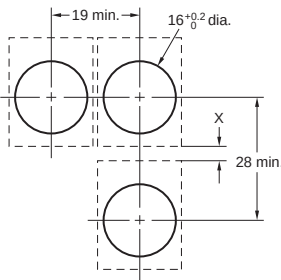
Panel Cutout (Top View)
