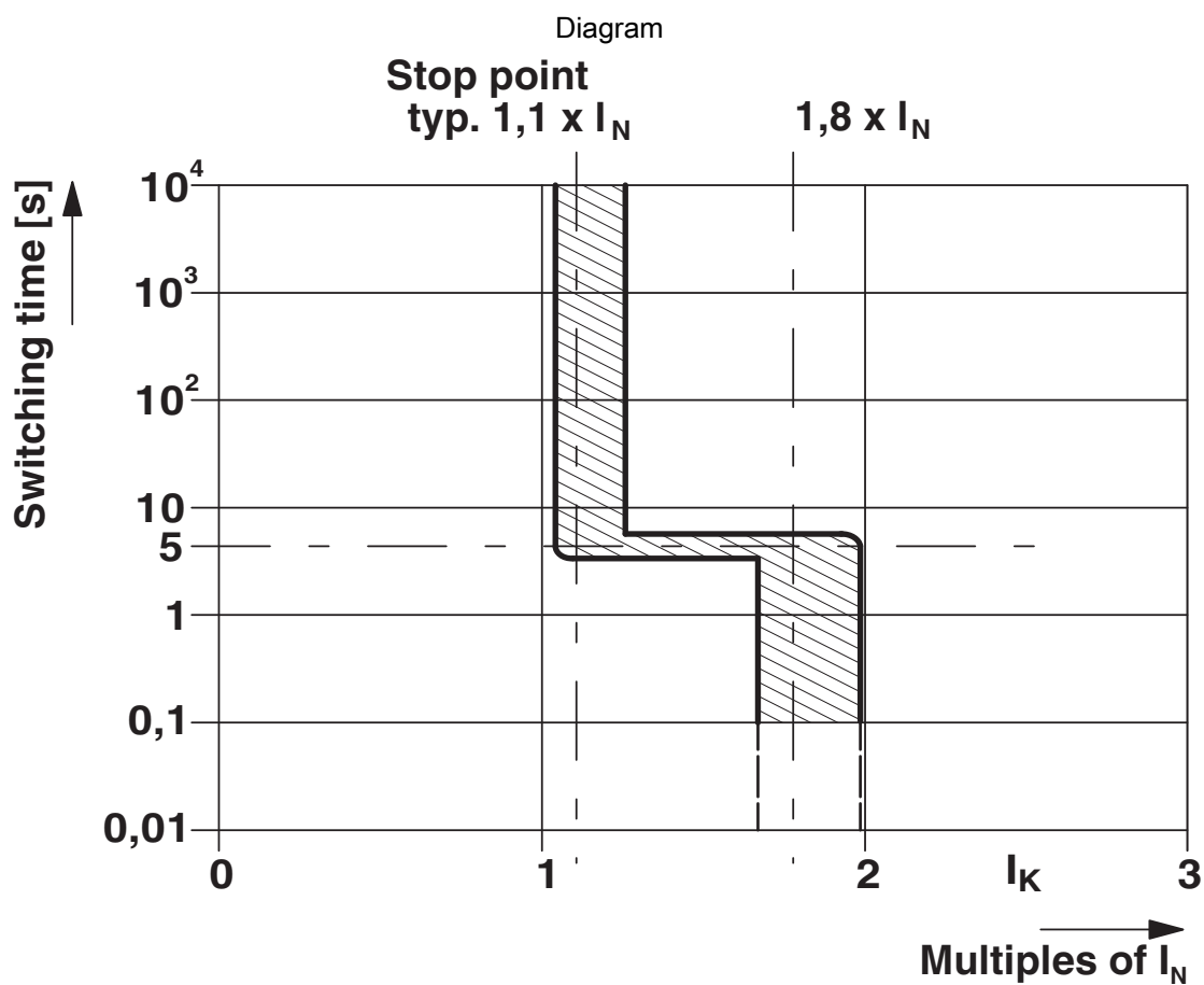
Trigger characteristic
