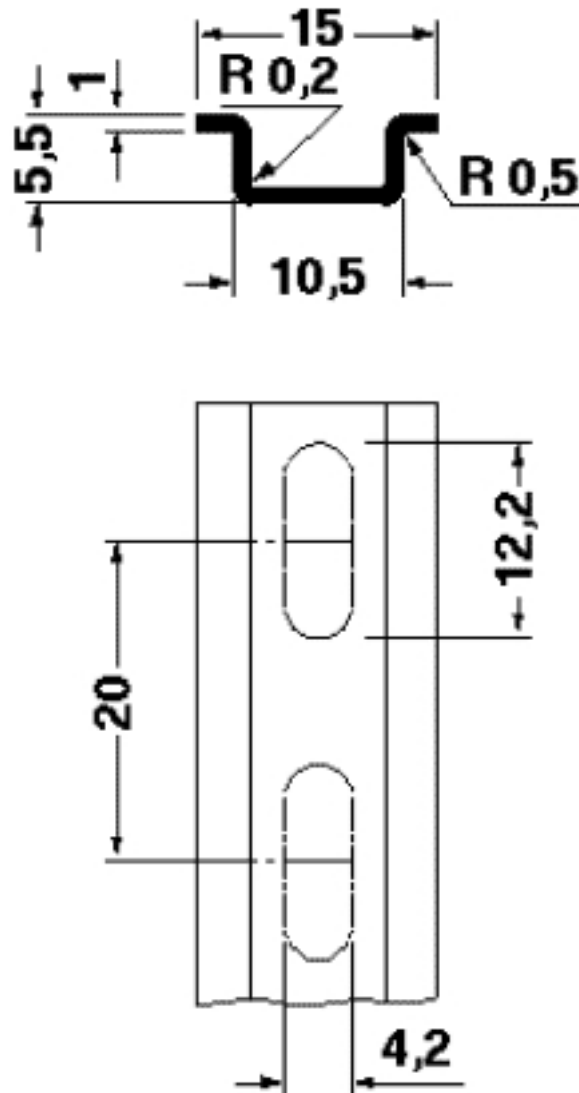
Dimensional drawing
