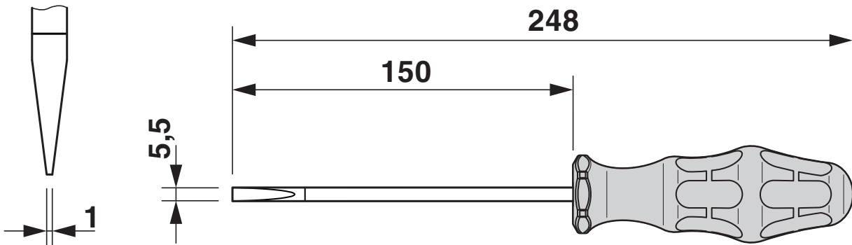
Dimensioned drawing
