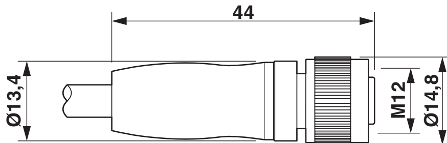
Dimensional drawing
