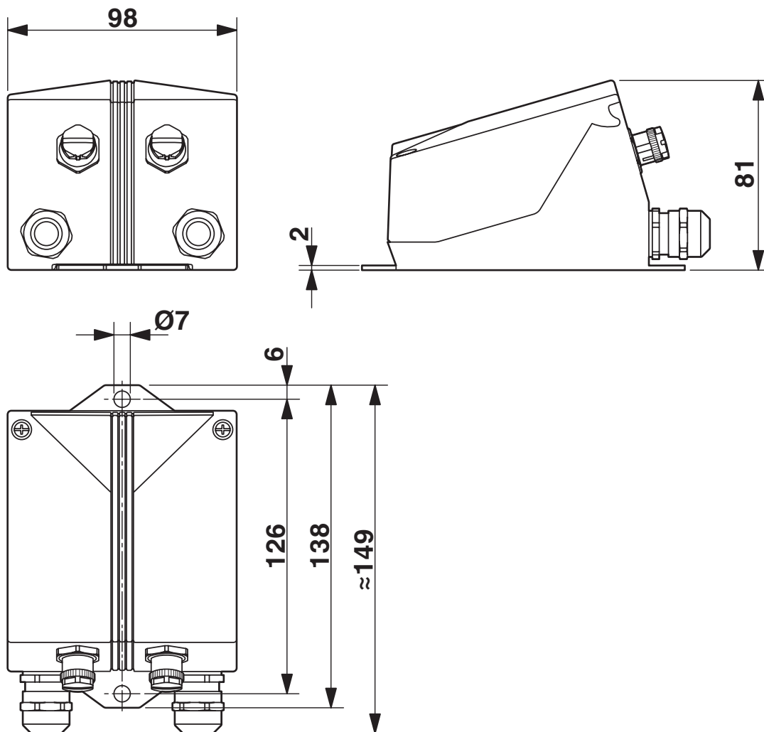
Dimensional drawing
