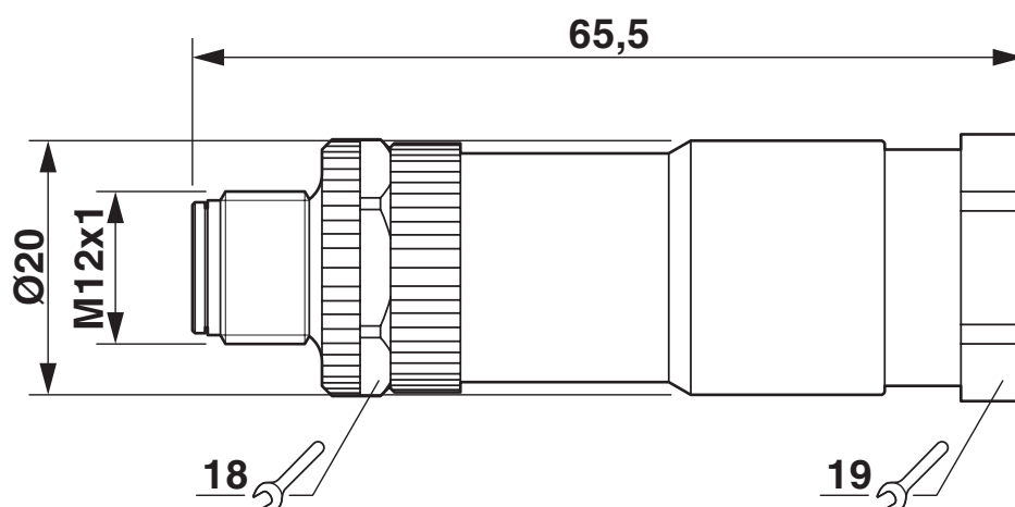
Dimensional drawing
