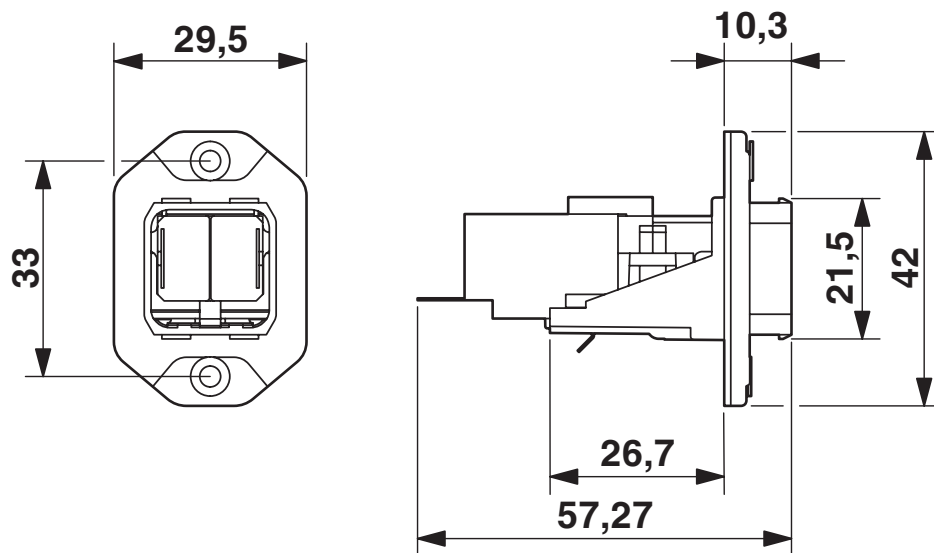
Push-Pull SC-RJ panel mounting frame
