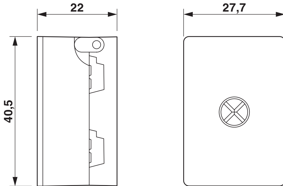
Dimensional drawing
