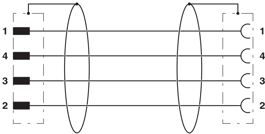
Circuit diagram
