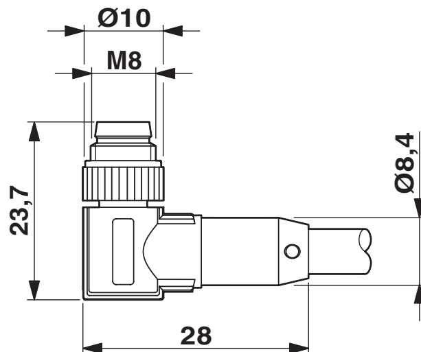
Dimensional drawing
