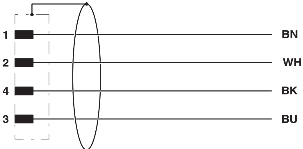
Circuit diagram
