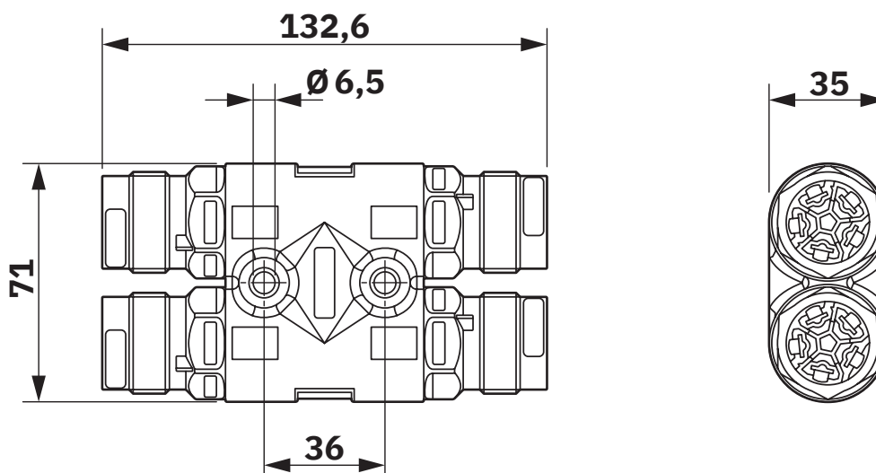
Dimensional drawing
