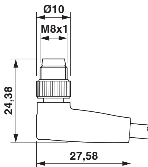
Dimensional drawing
