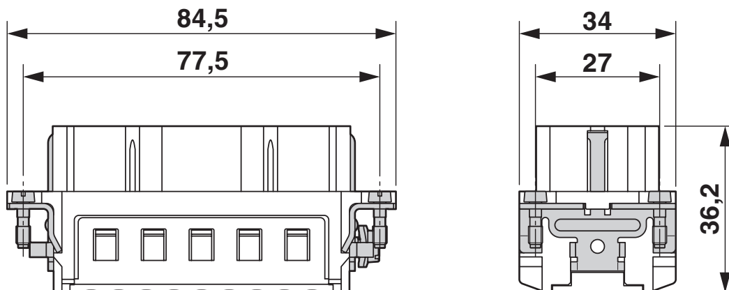
Dimensional drawing
