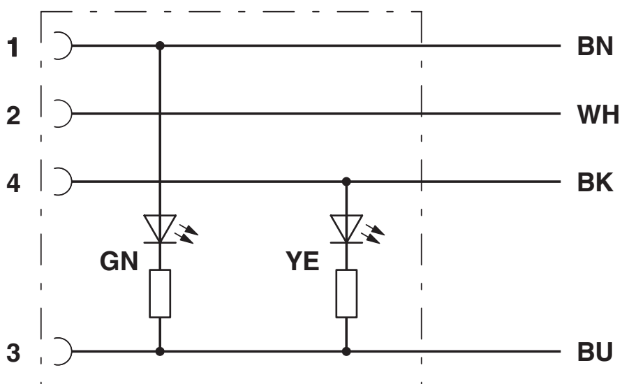
Circuit diagram
