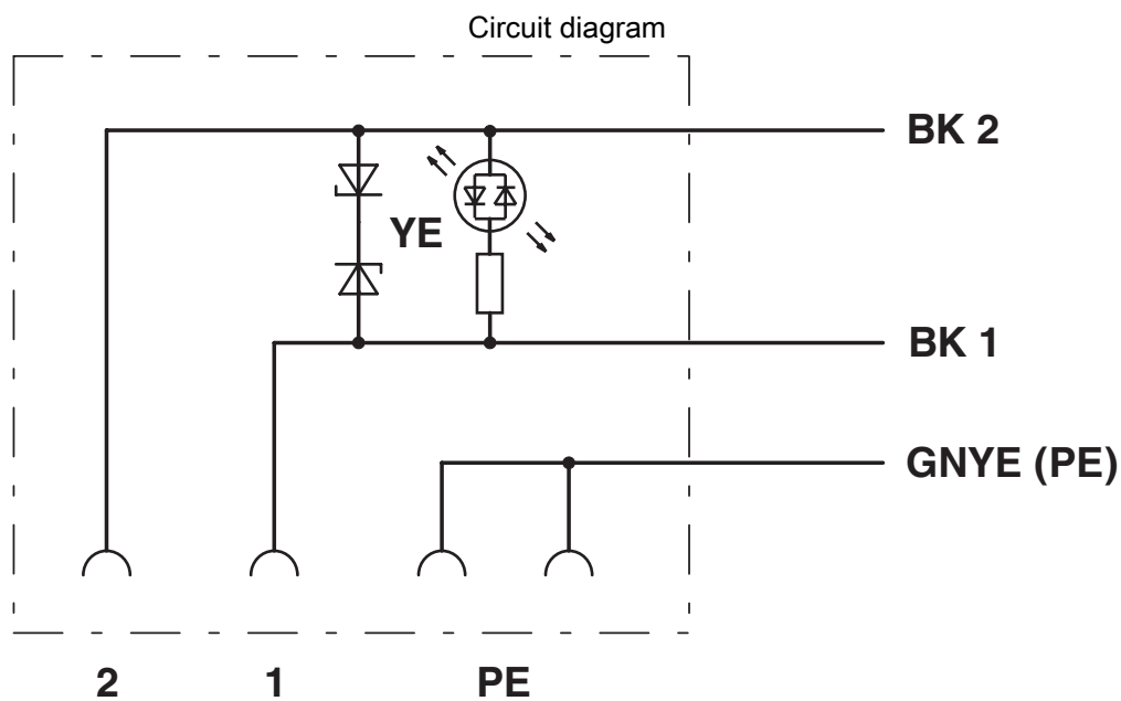
Valve connector, type A, side view
