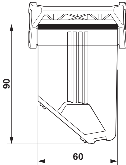
Dimensional drawing
