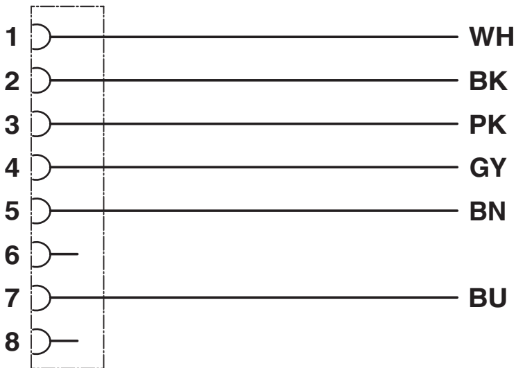
Circuit diagram
