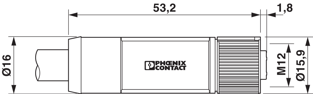
Dimensional drawing
