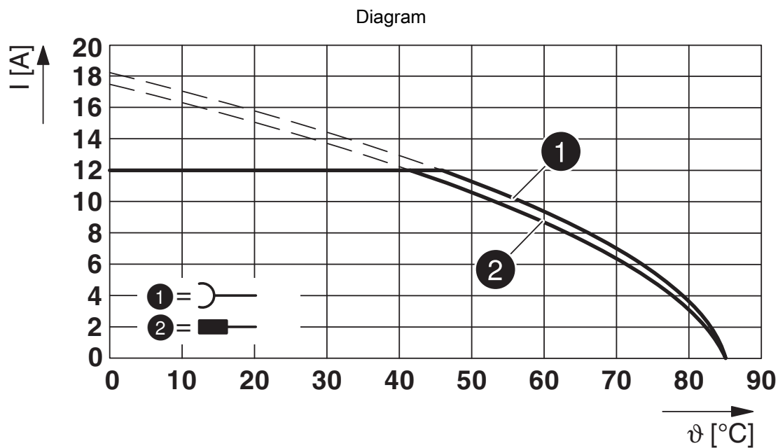
Schematic diagram
