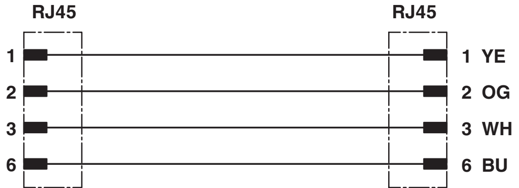
Circuit diagram
