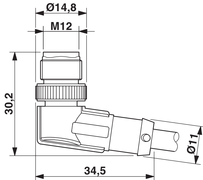
Dimensional drawing
