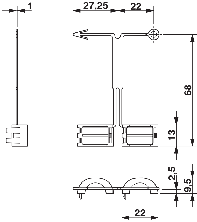
Dimensional drawing
