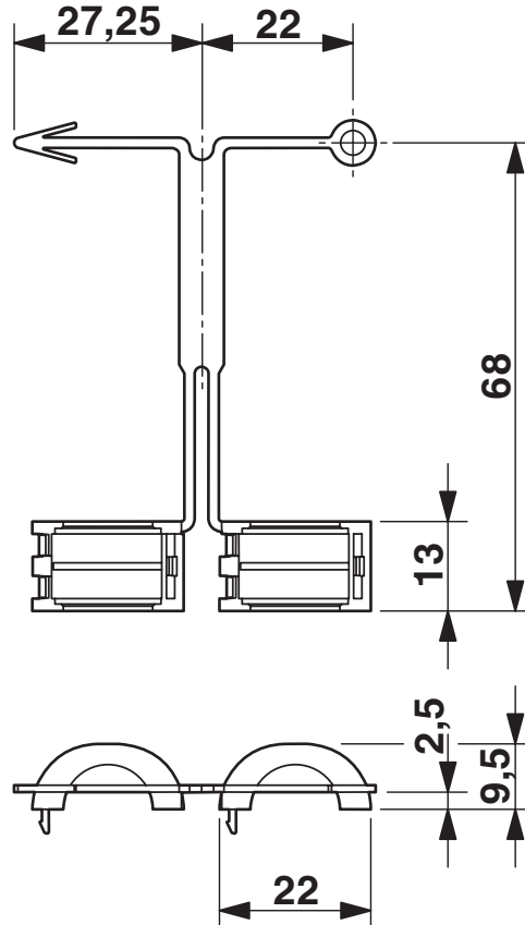
Dimensional drawing
