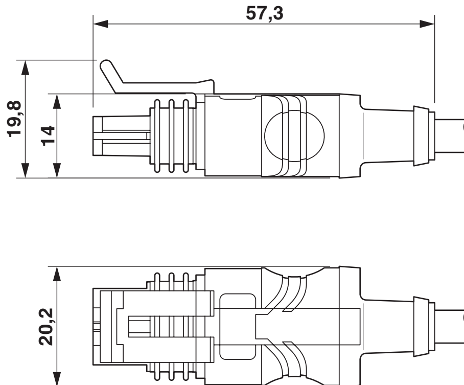
Dimensional drawing
