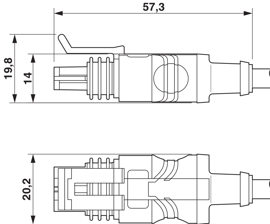
Dimensional drawing
