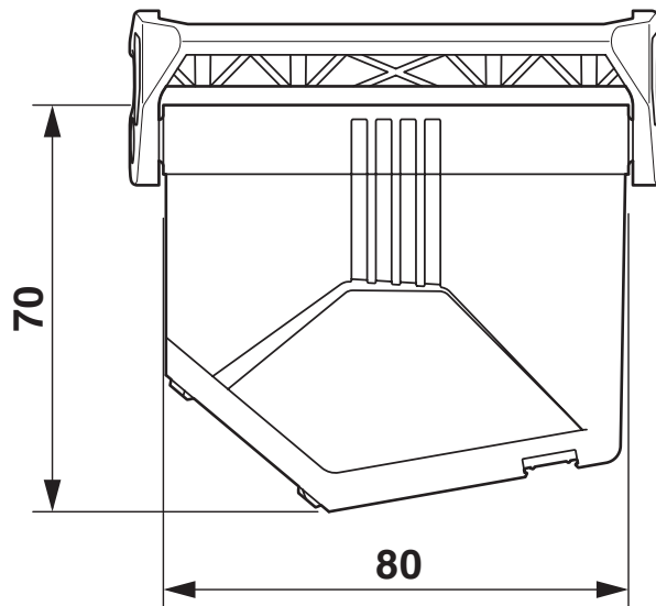
Dimensional drawing
