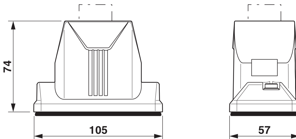
Dimensional drawing
