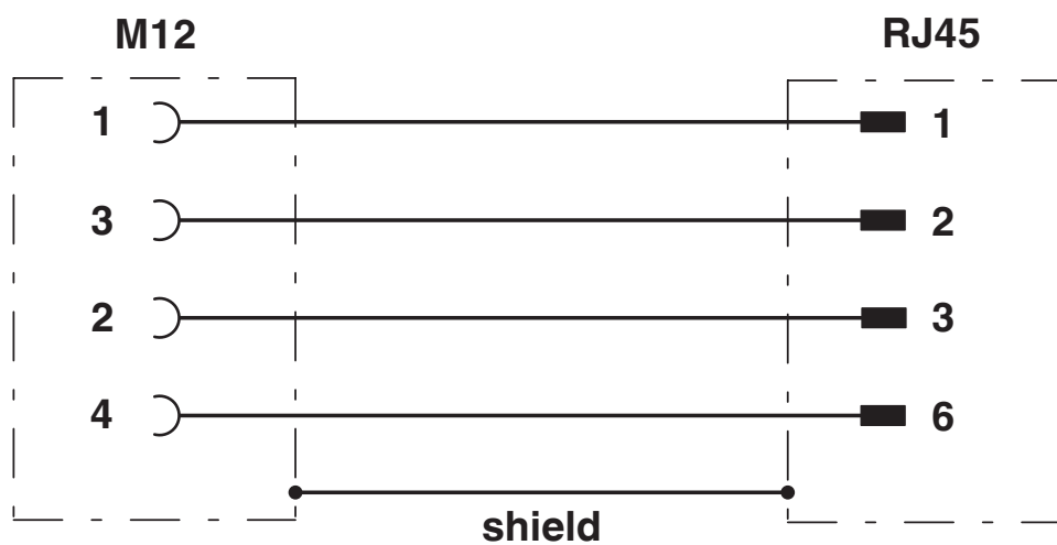
Circuit diagram
