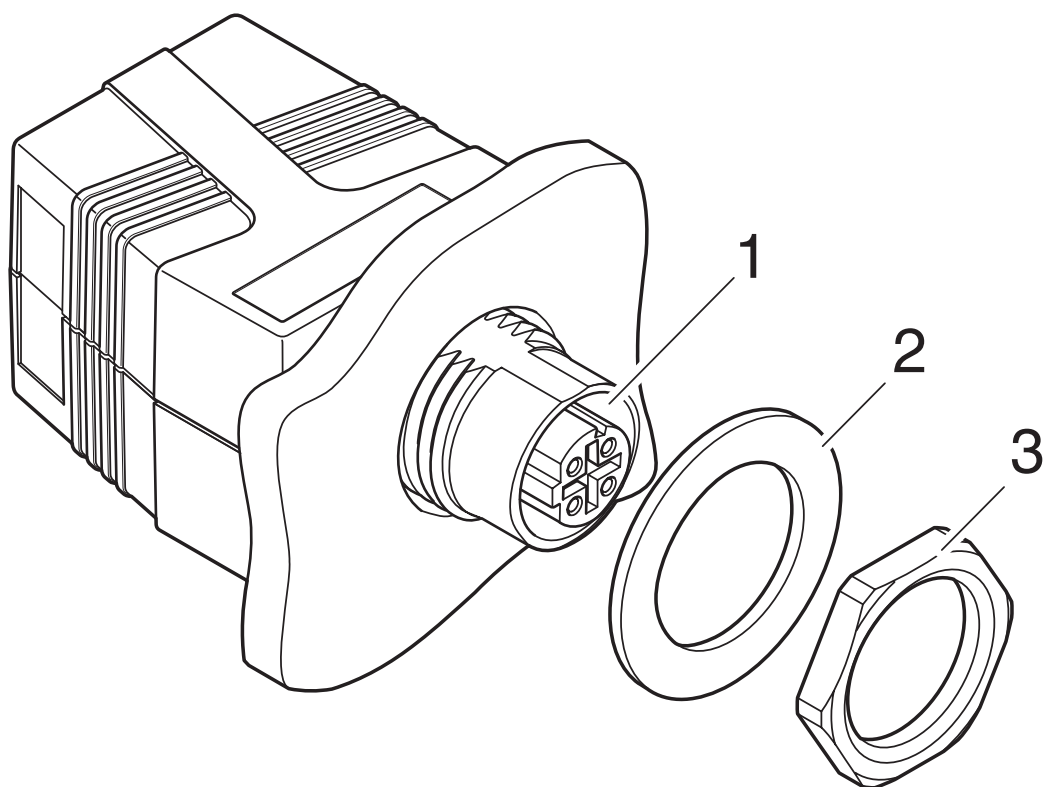
Exploded view
