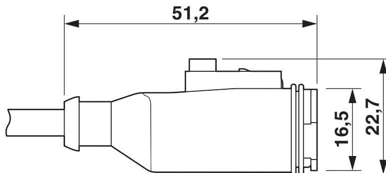
Dimensional drawing
