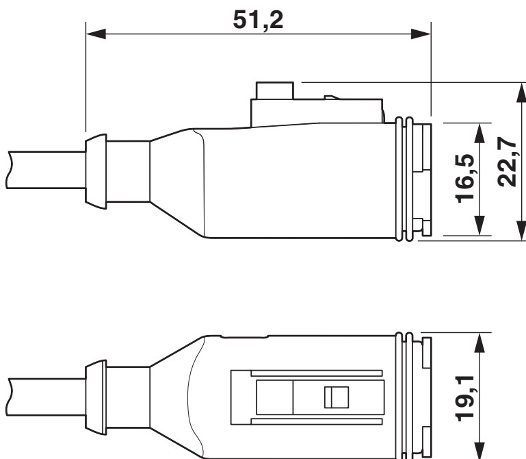
Dimensional drawing
