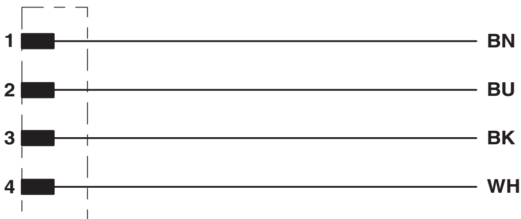
Circuit diagram
