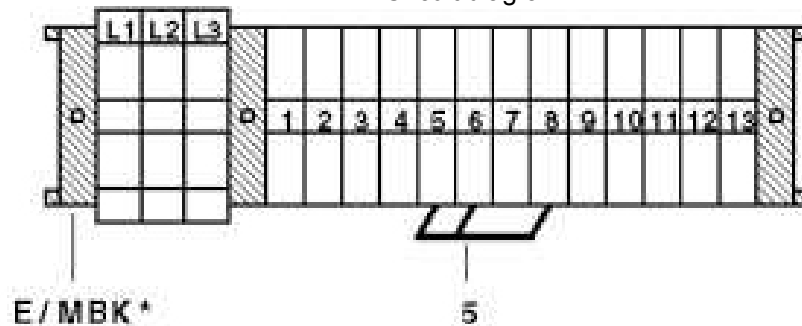
Circuit diagram
