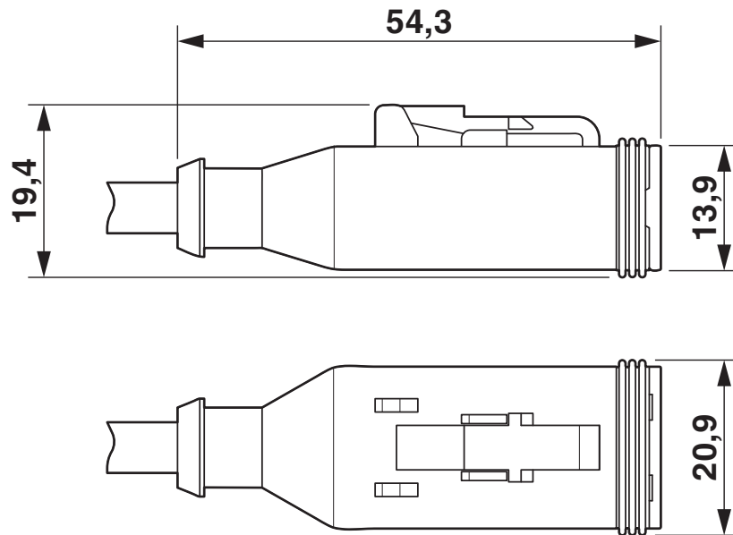
Dimensional drawing
