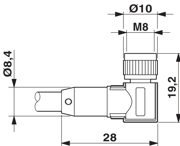
Dimensional drawing
