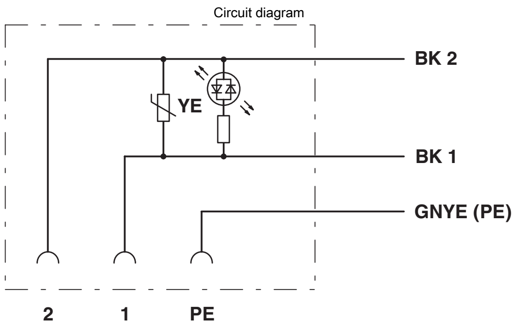
Valve connector pin assignment, type B
