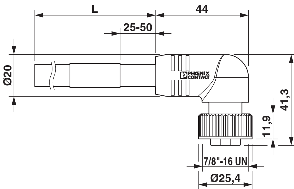
Dimensional drawing
