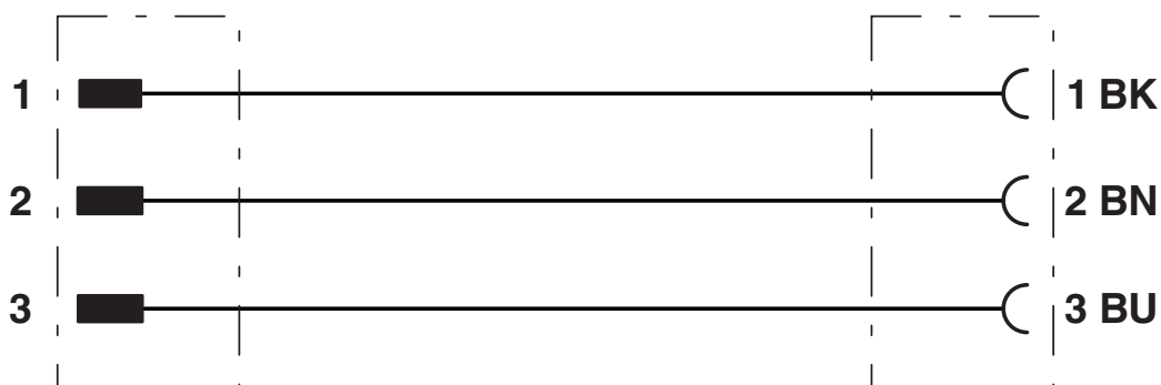
Circuit diagram
