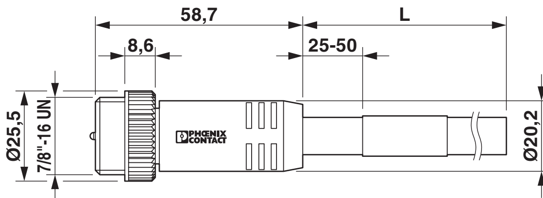
7/8"-16UNF plug, straight
