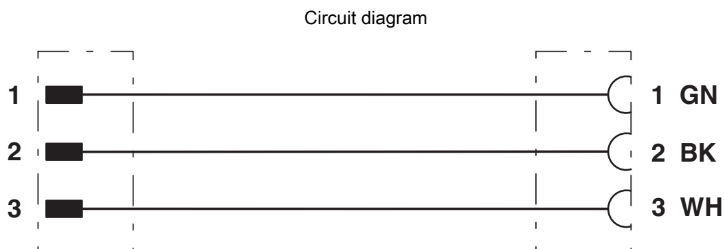
Pin assignment, plug, 7/8"-16UNF, 3-pos., view of male side
