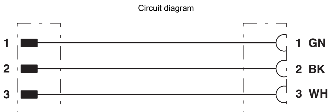
Pin assignment, plug, 7/8"-16UNF, 3-pos., view of male side
