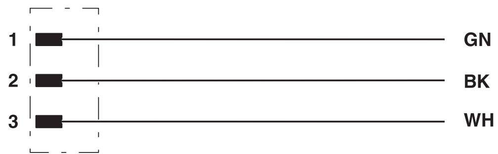
Circuit diagram
