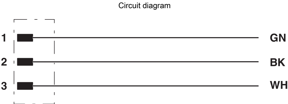
Pin assignment, plug, 7/8"-16UNF, 3-pos., view of male side
