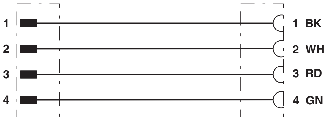
Circuit diagram
