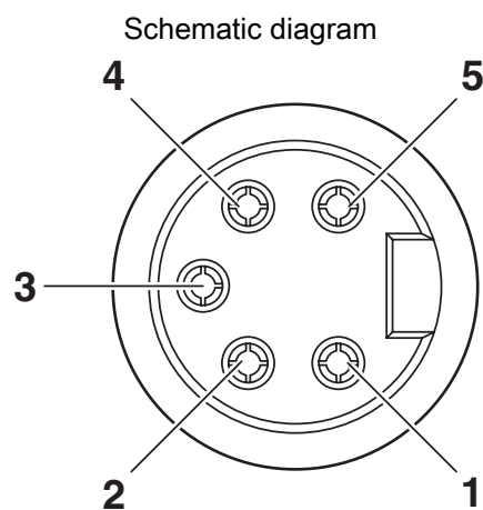
Circuit diagram
