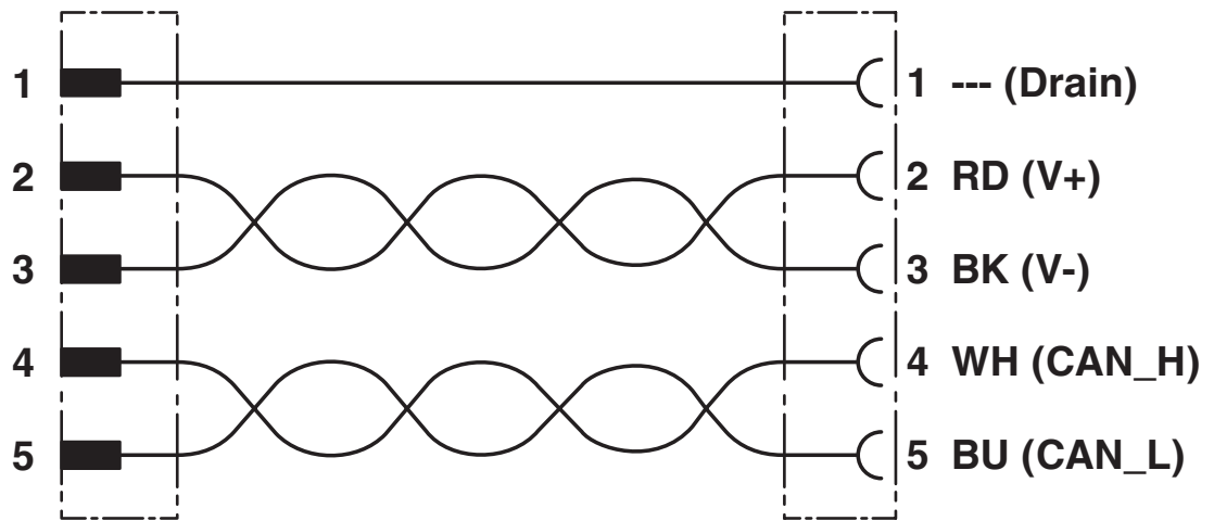
Circuit diagram
