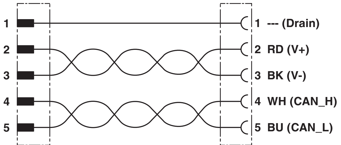
Circuit diagram
