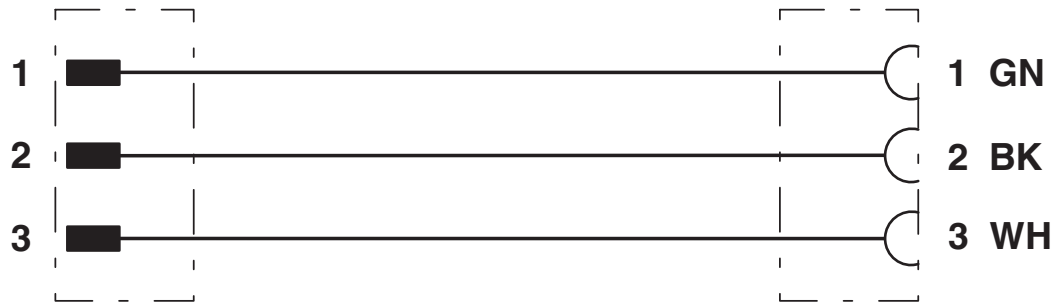
Circuit diagram
