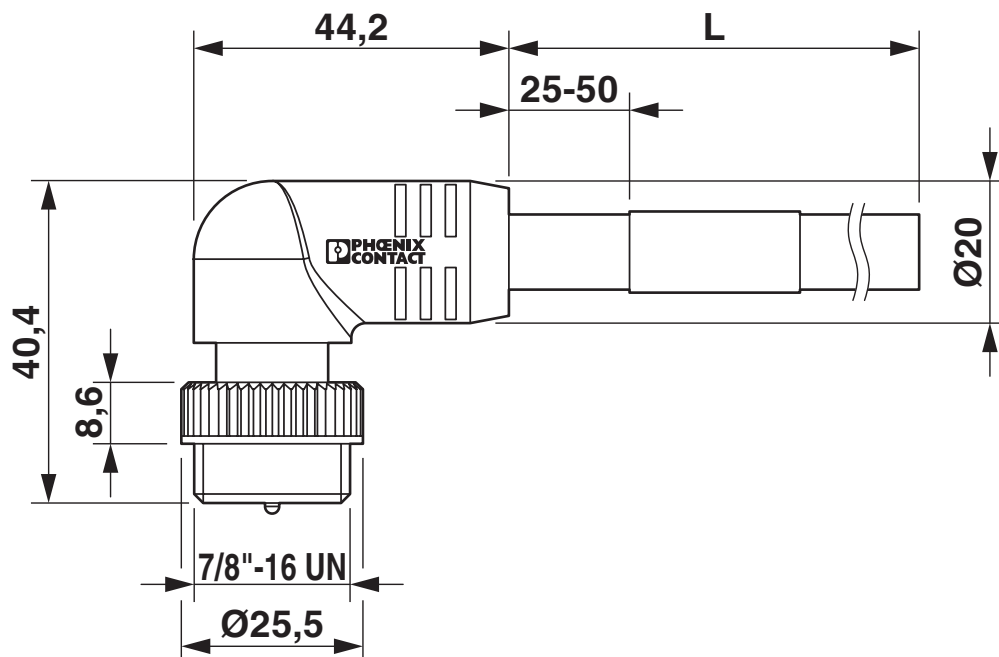
Dimensional drawing
